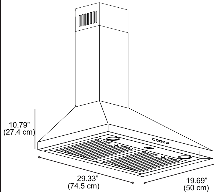
Dimension of: OV-2002 / OV-2022
